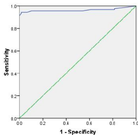
ROC Curve
